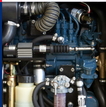
1800 rpm Kubota engine
